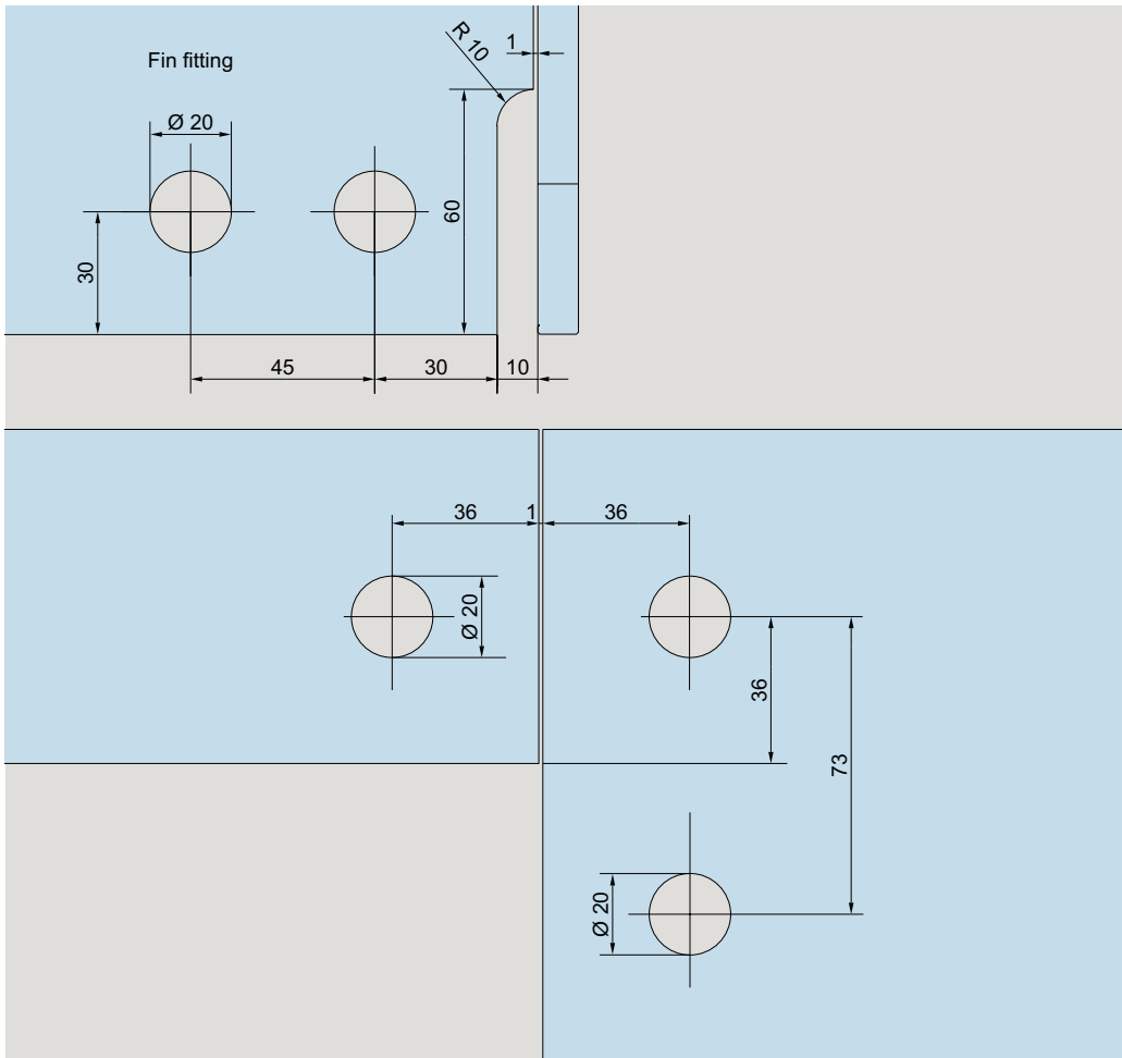
PT 61 Single overpanel connector with fin fitting inside
